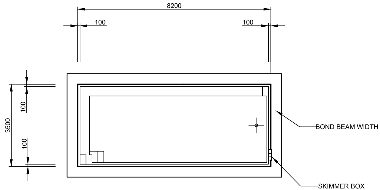
PLAN VIEW SCALE 1 : 100
